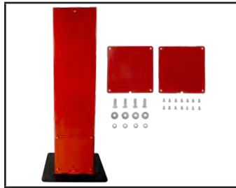
Pedestal Kit Pedestal to be used with only FR902DPU and FR302DPU UPC# 089404224540
