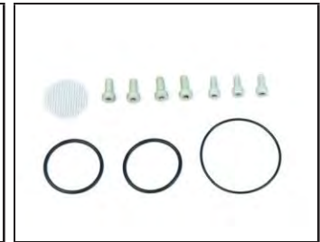
Seal Kit Rotor cover gasket, flange o-rings (2), flange screws (4), rotor cover screws (3), inlet screen UPC# 089404224816
