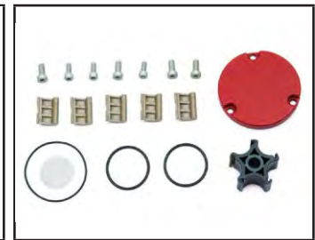
12 GPM Rebuild Kit Rotor, rotor cover, flange screws (4), inlet screen, vanes (5), rotor cover gasket, rotor cover screws (3), flange o-rings (2) UPC# 089404225097
